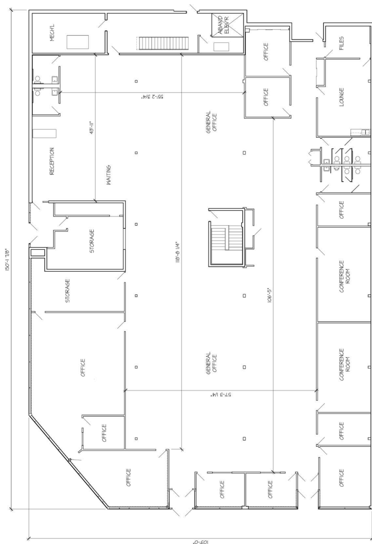
Existing Conditions - Main Floor Plan
