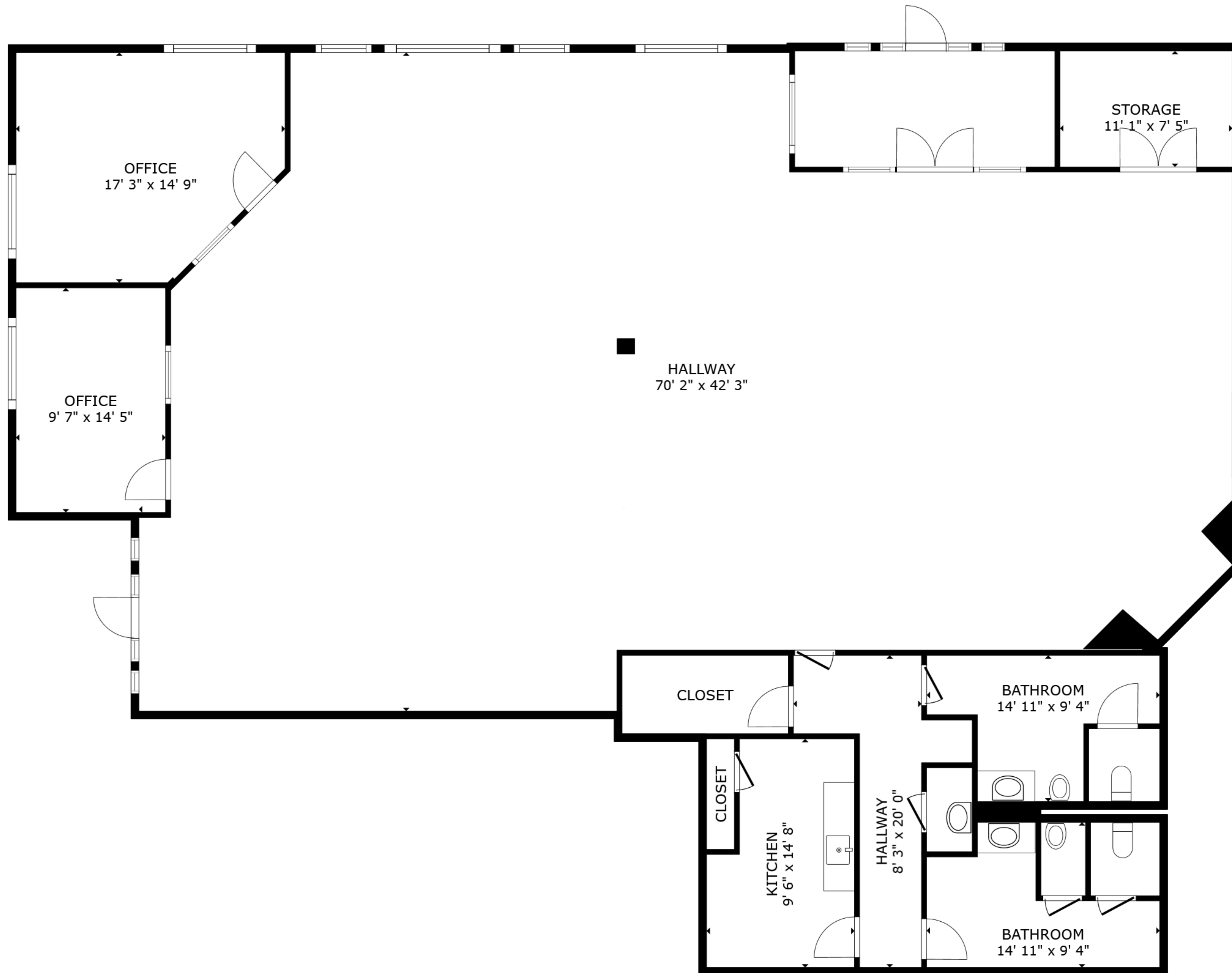
FLOOR PLAN
