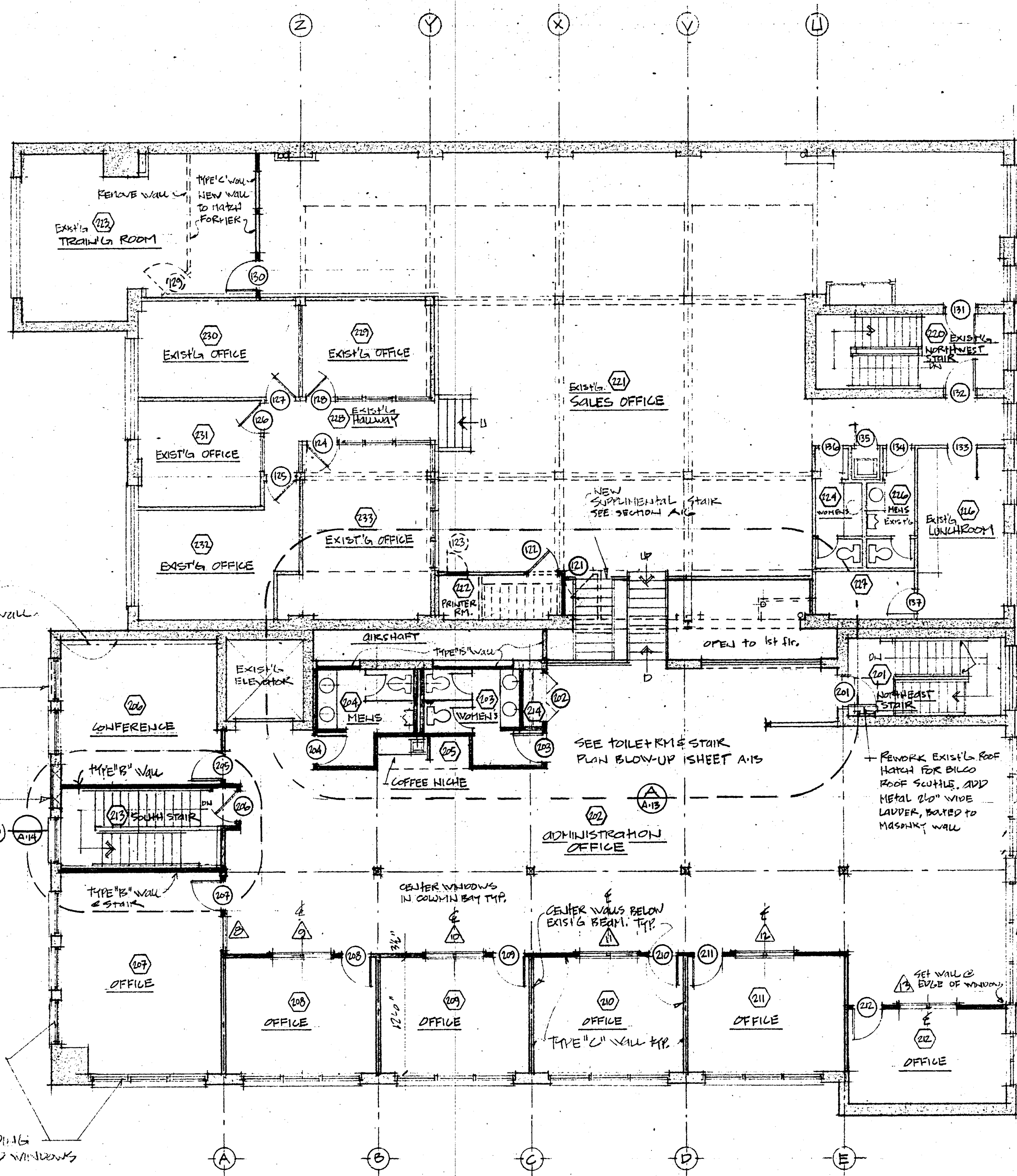
SECOND FLOOR 1/8" = 1'-0"
