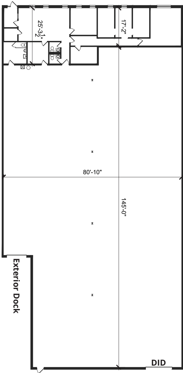
FLOOR PLAN
