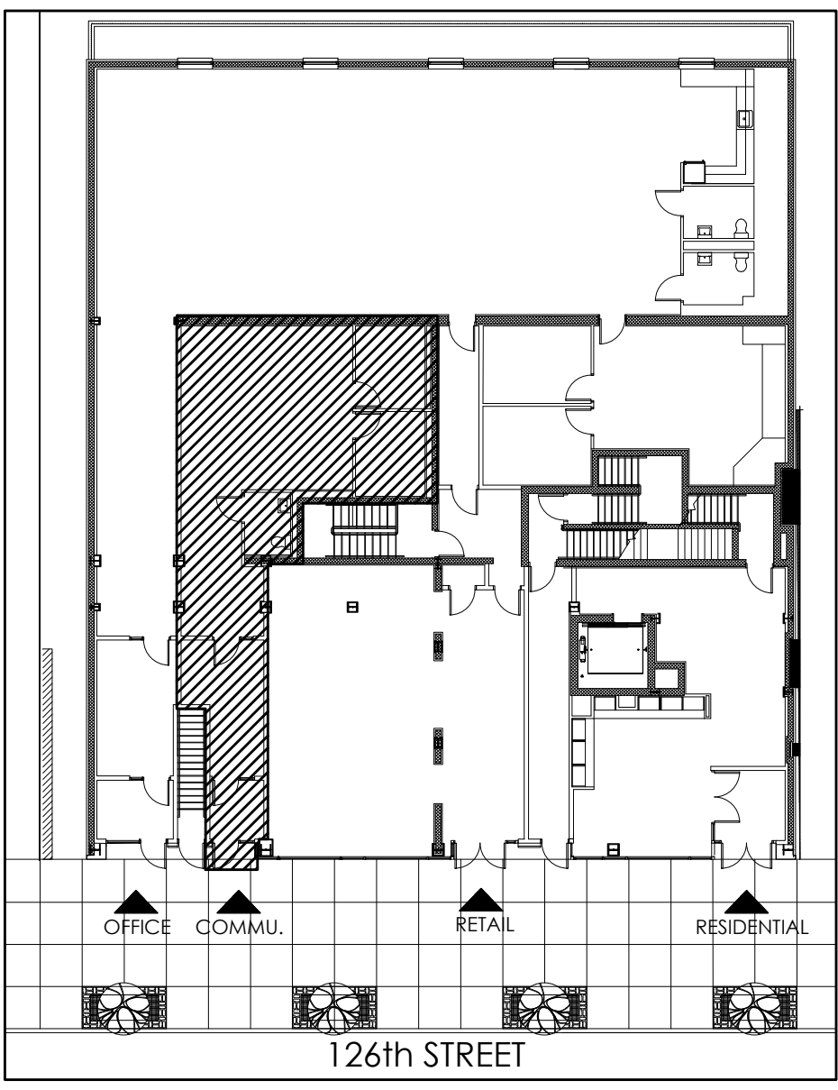
LOCATION PLAN N SCALE : OUT OF SCALE
