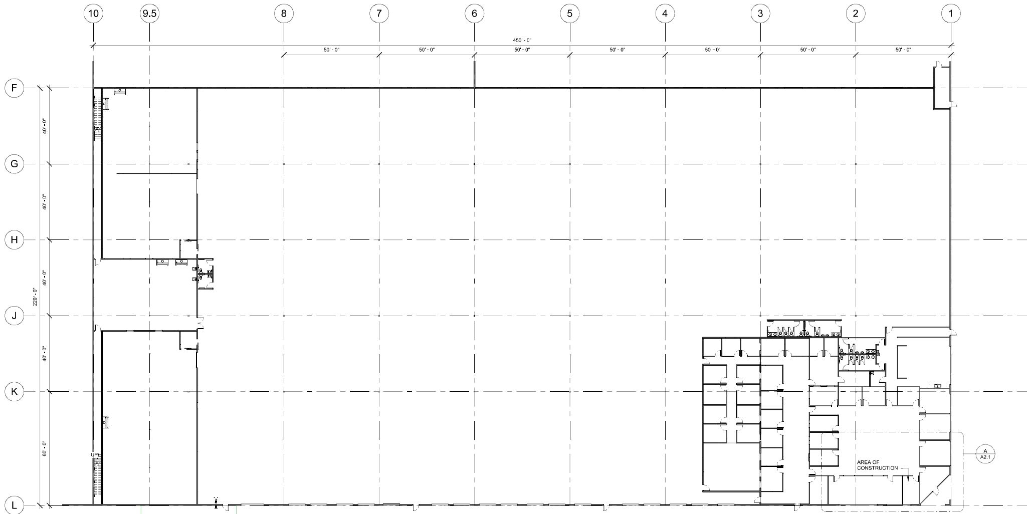
OVERALL FLOOR PLAN 1" = 20'-0"
