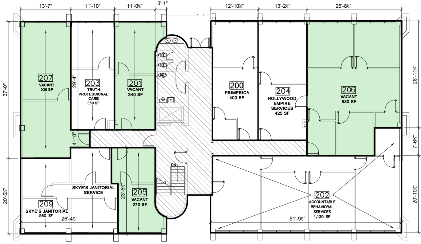
Available Suites Common Areas 7240 CROWDER BLVD: 2ND FLOOR SCALE: 1/16" = 1'-0"
