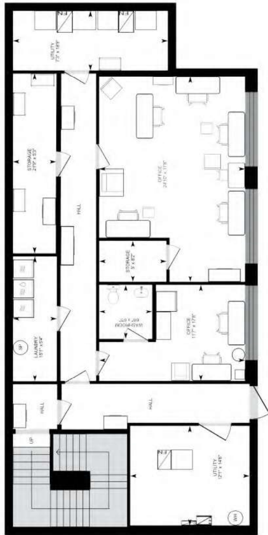
Basement/Lower Level
