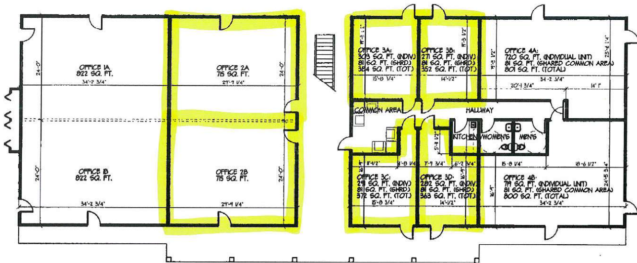
First Floor Plan, 1/16"=1'-0" North ☐ 6144 Sq. Ft. Office Space
