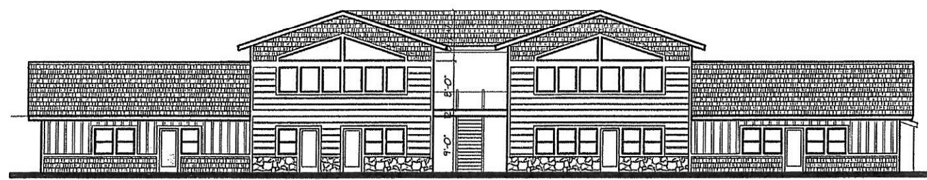
West Elevation, 1/16"=1'-0"
