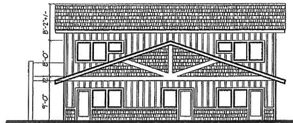
North Elevation, 1/16"=1'-0"
