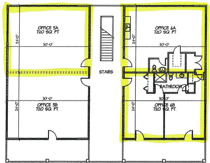
Second Floor Plan, 1/16"=1'-0" North ⬤ 2880 Sq. Ft. Office Space
