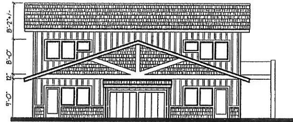
South Elevation, 1/16"=1'-0"
