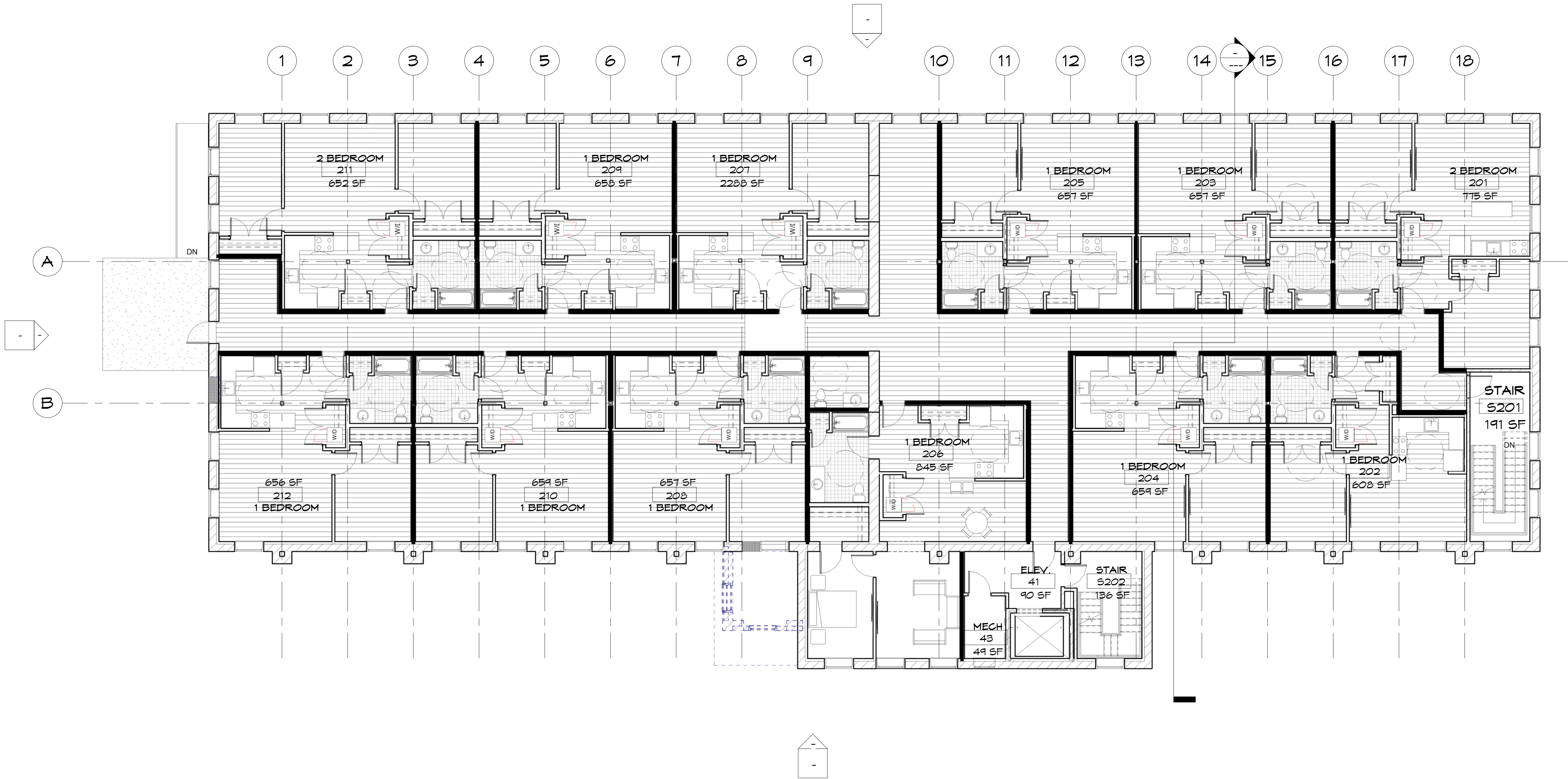
1 SECOND FLOOR 1/8" = 1'-0"
