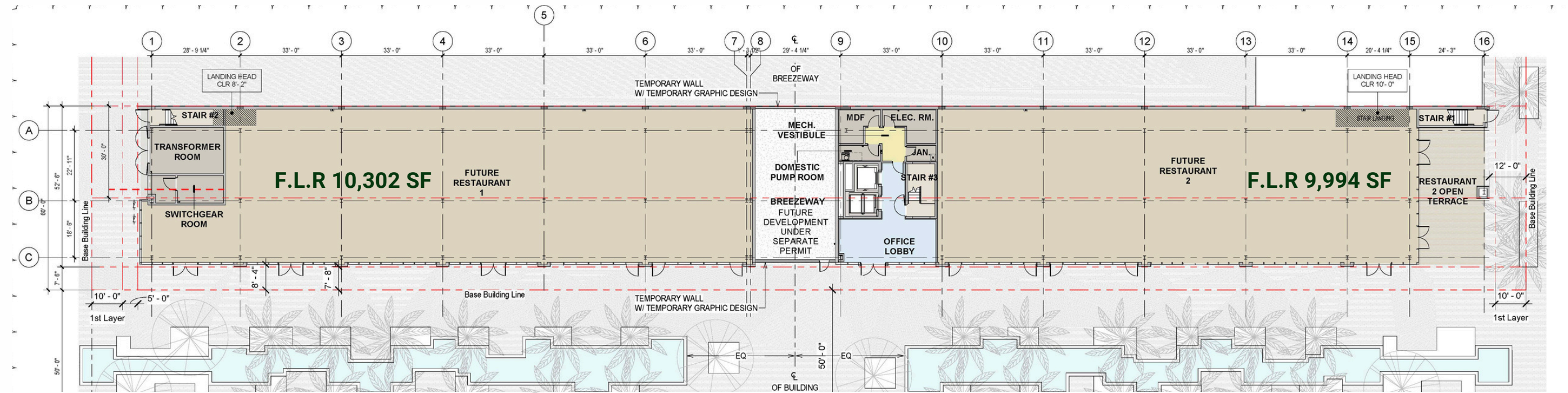
Ground Floor
