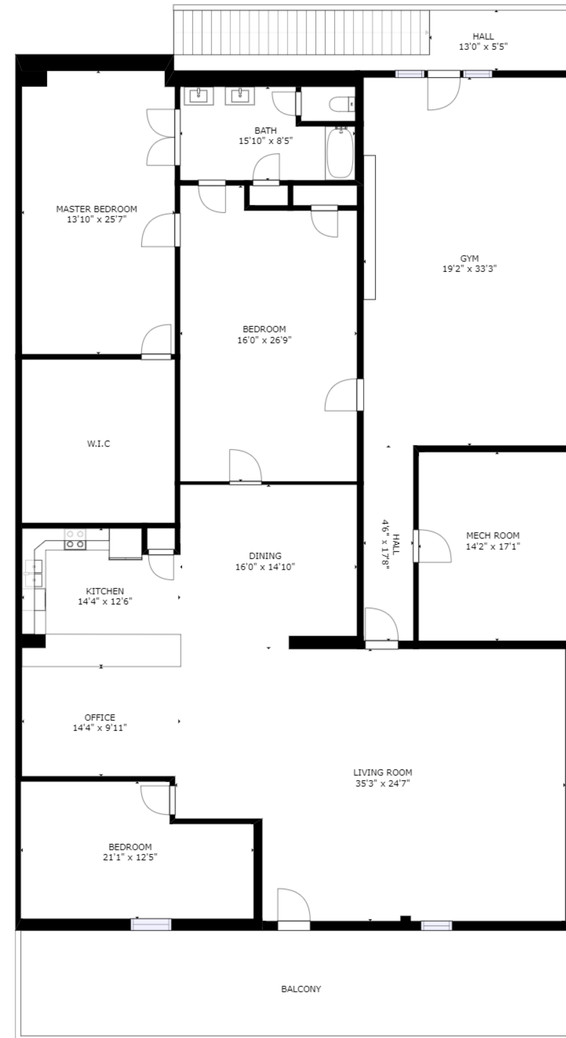
FLOOR 2
