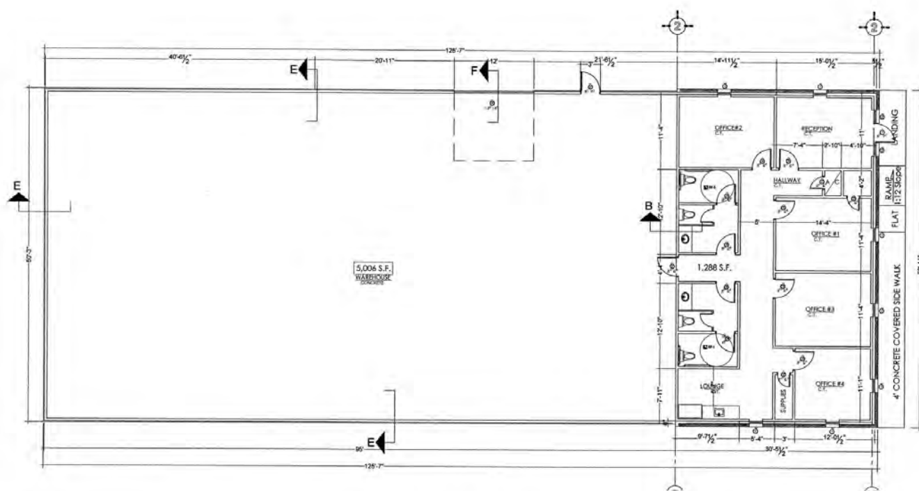
FLOOR PLAN
