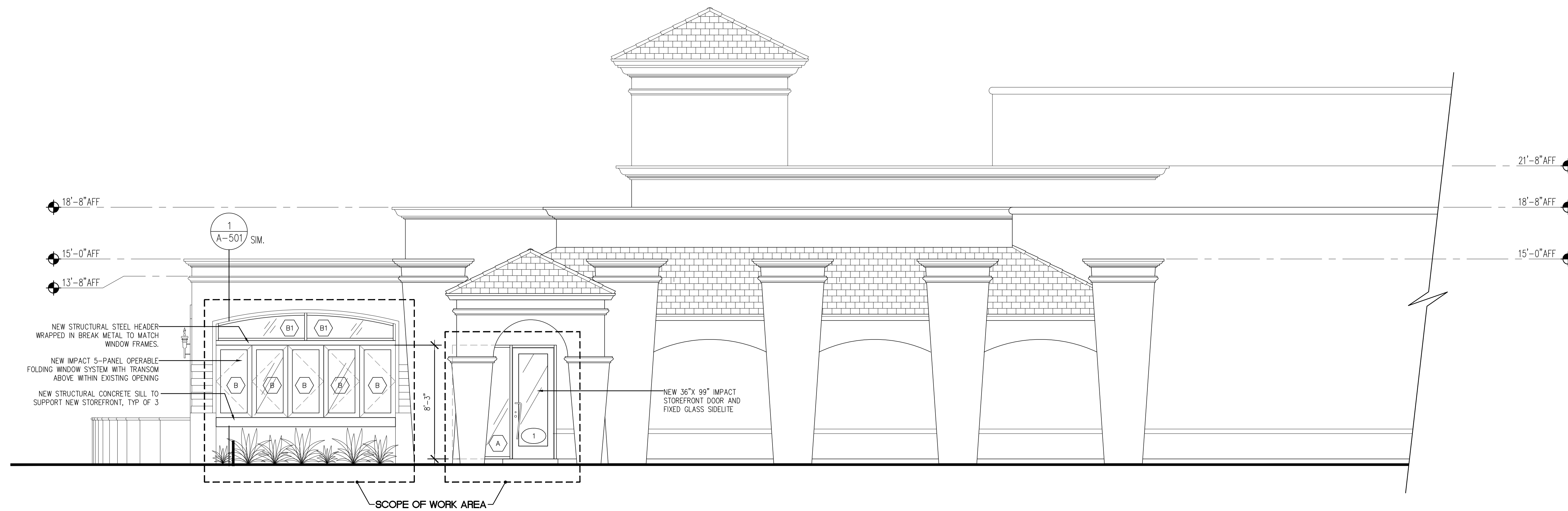
PROPOSED SOUTH ELEVATION 1/4" = 1'-0" 2
