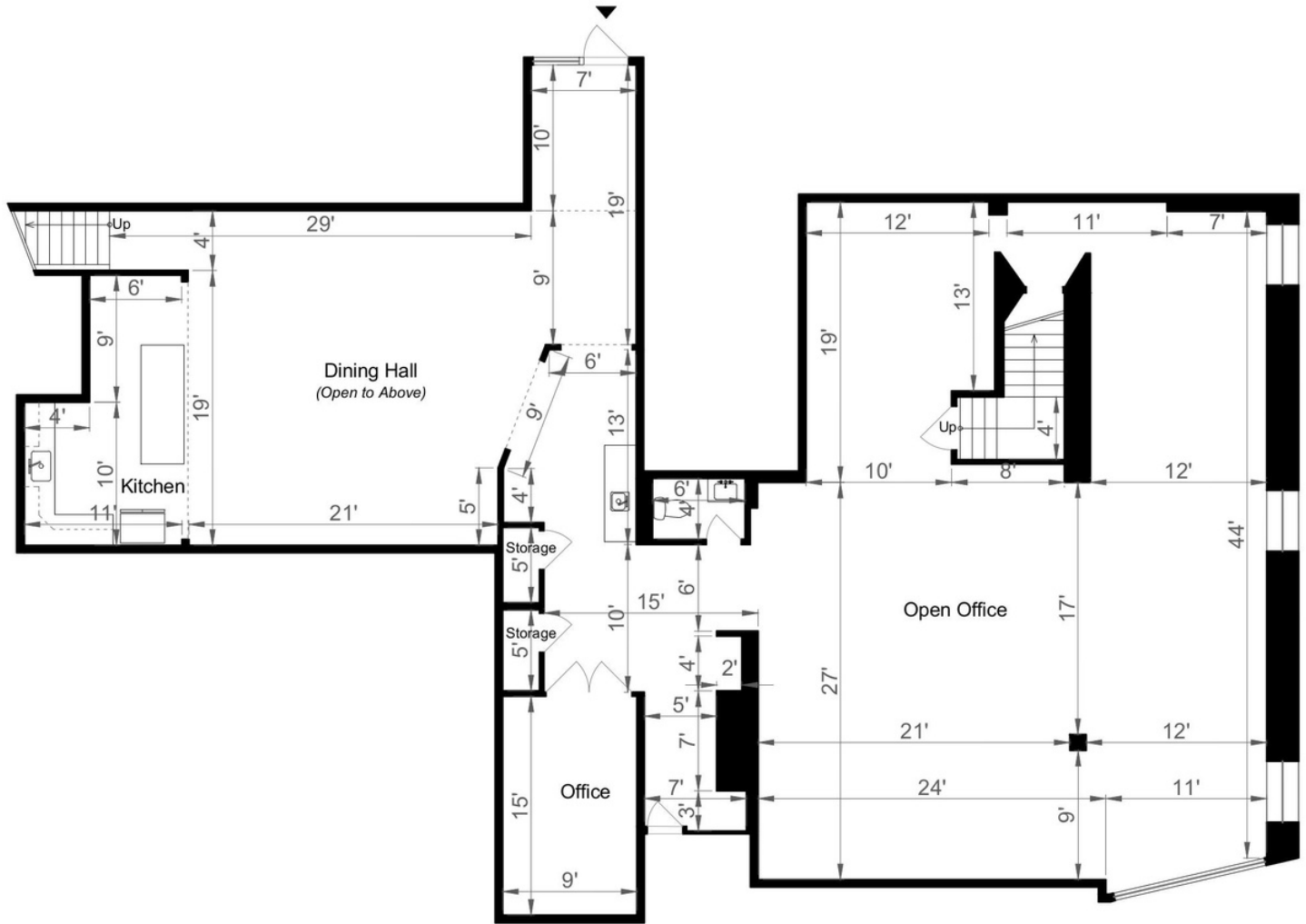
FIRST FLOOR 3,145 SQ FT
