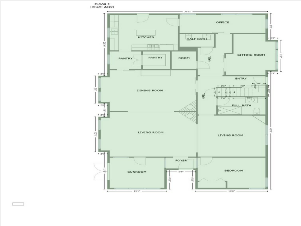
Floor Plan Main Level
