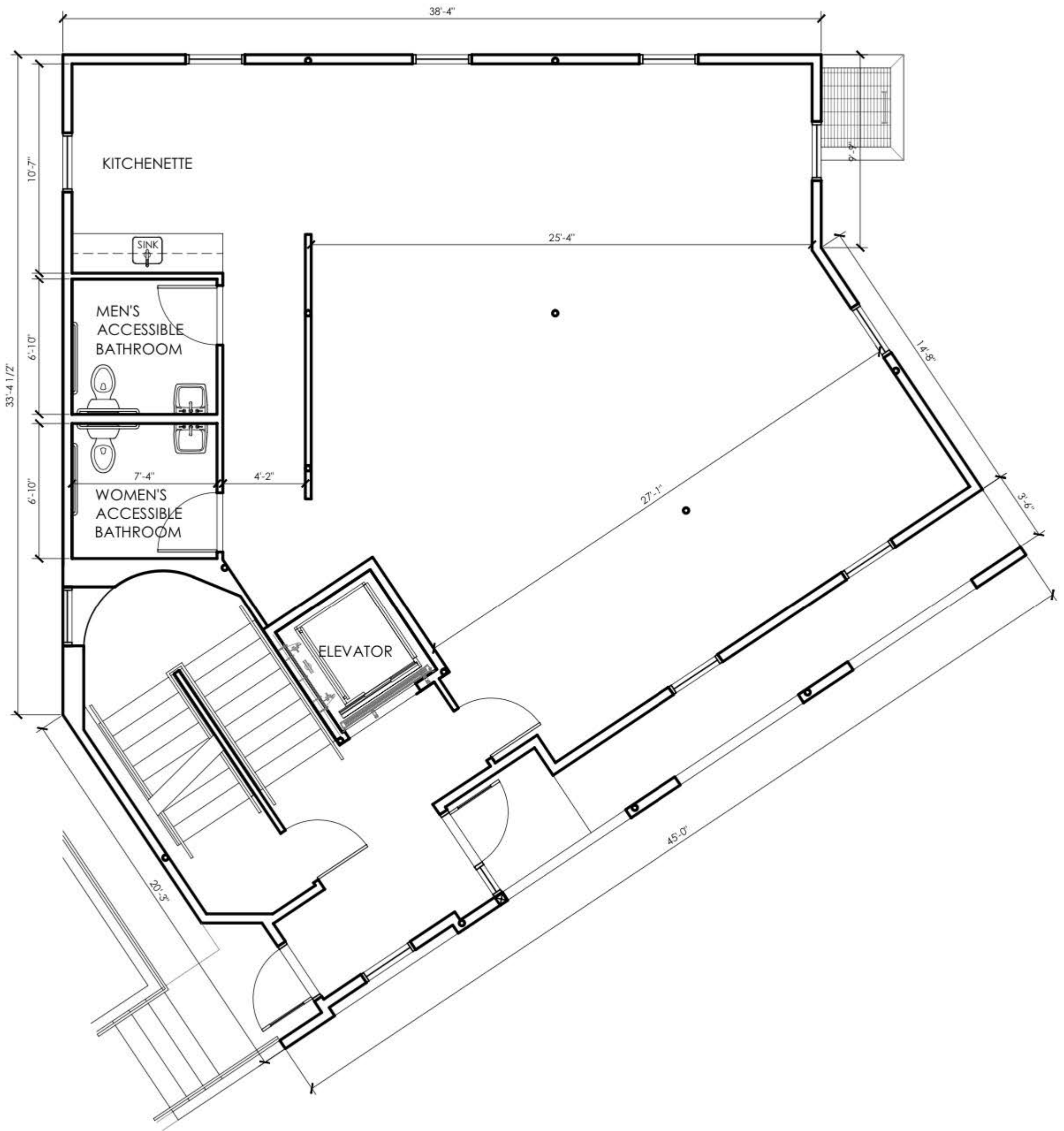
② FIRST FLOOR CONSTRUCTION PLAN 1/8" = 1'
