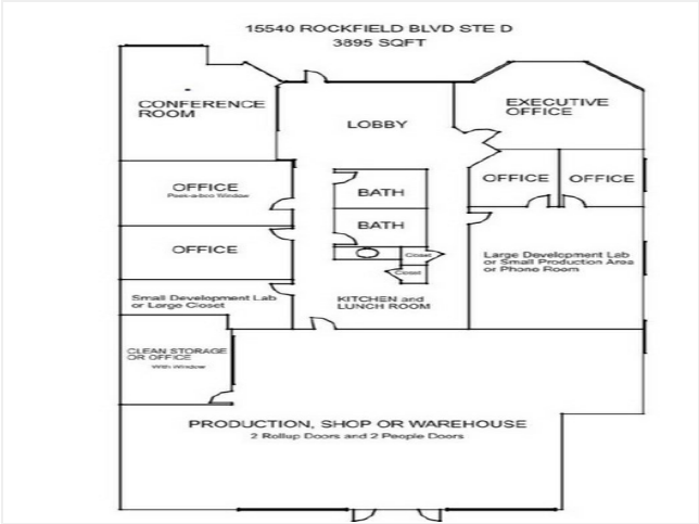
Rockfield Floorplan 250212
