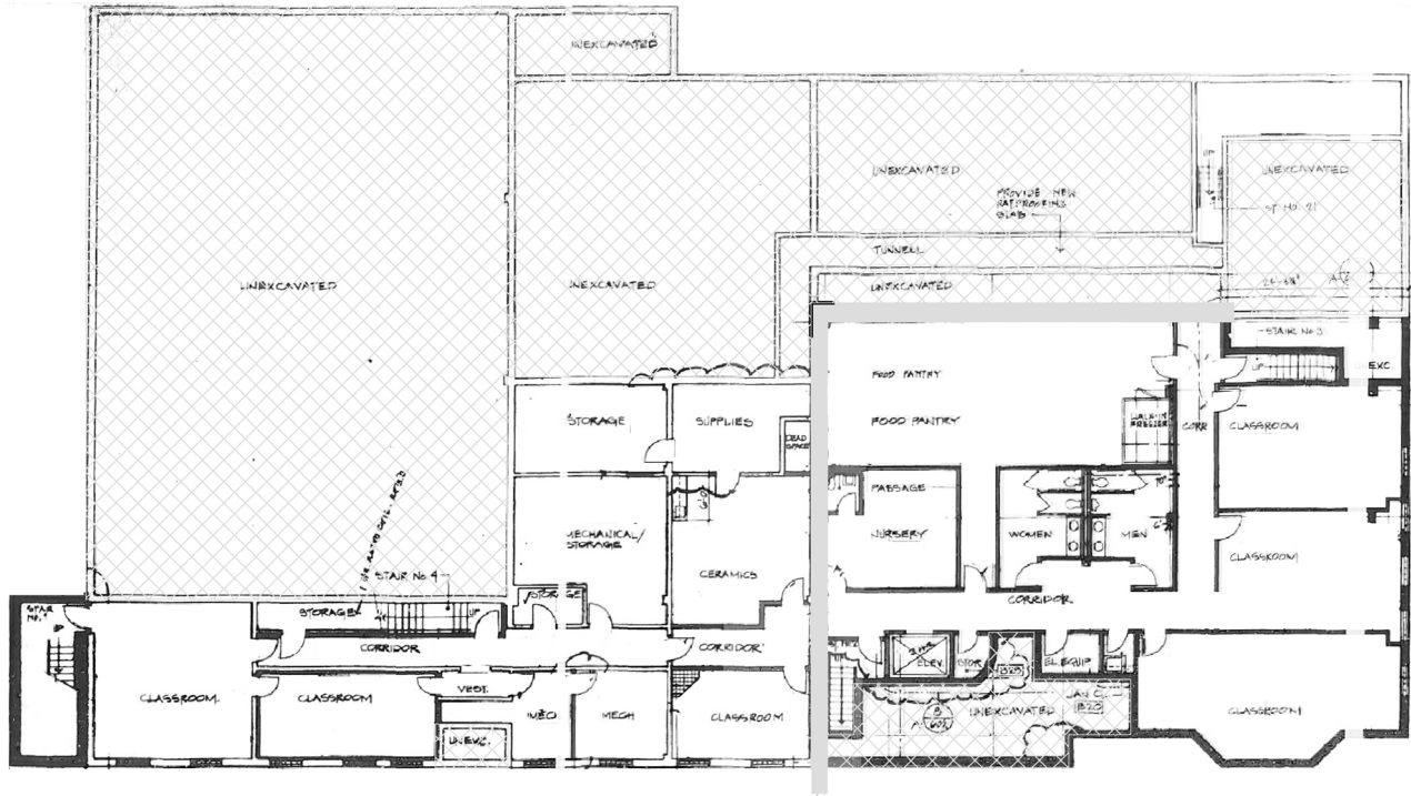
LOWER LEVEL FLOOR PLAN
