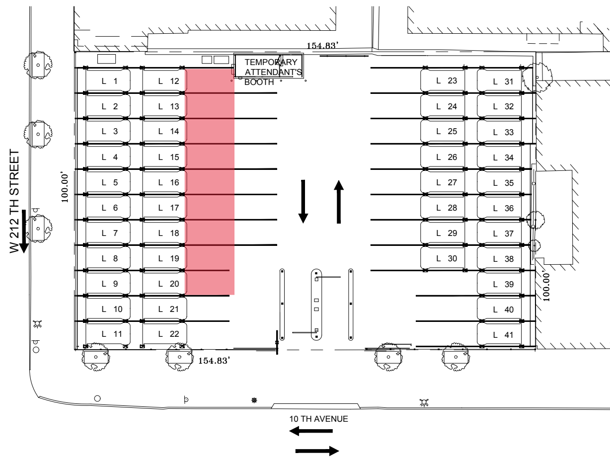
CURRENT PARKING PLAN 1/32" = 1'-0"
