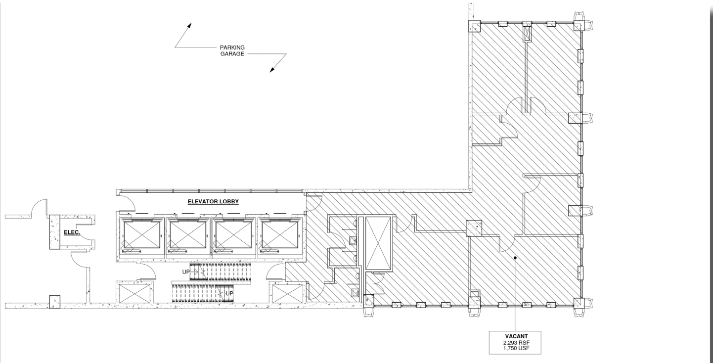
Typical Floor Plate - Floors 3-7
