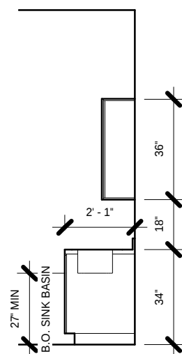
2 KITCHENETTE SECTION 1/4" = 1'-0"
