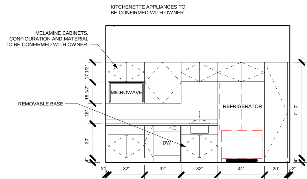
1 KITCHENETTE ELEVATION 1/4" = 1'-0"
