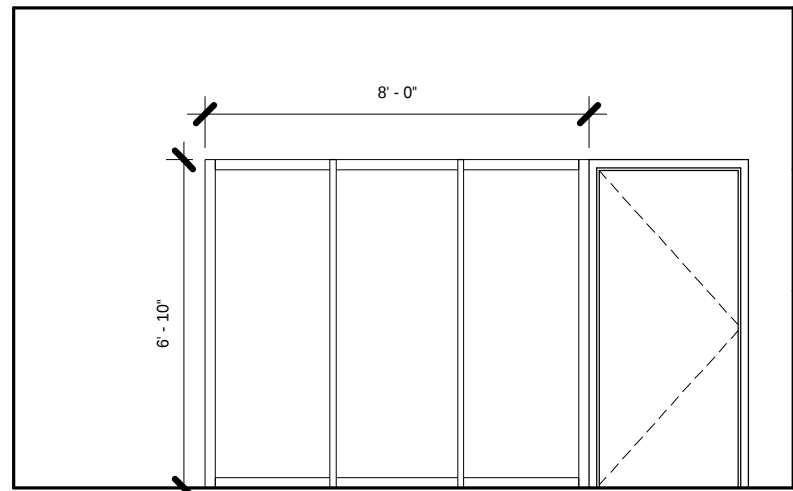
4 CONFERENCE ROOM WINDOW ELEVATION 1/4" = 1'-0"
