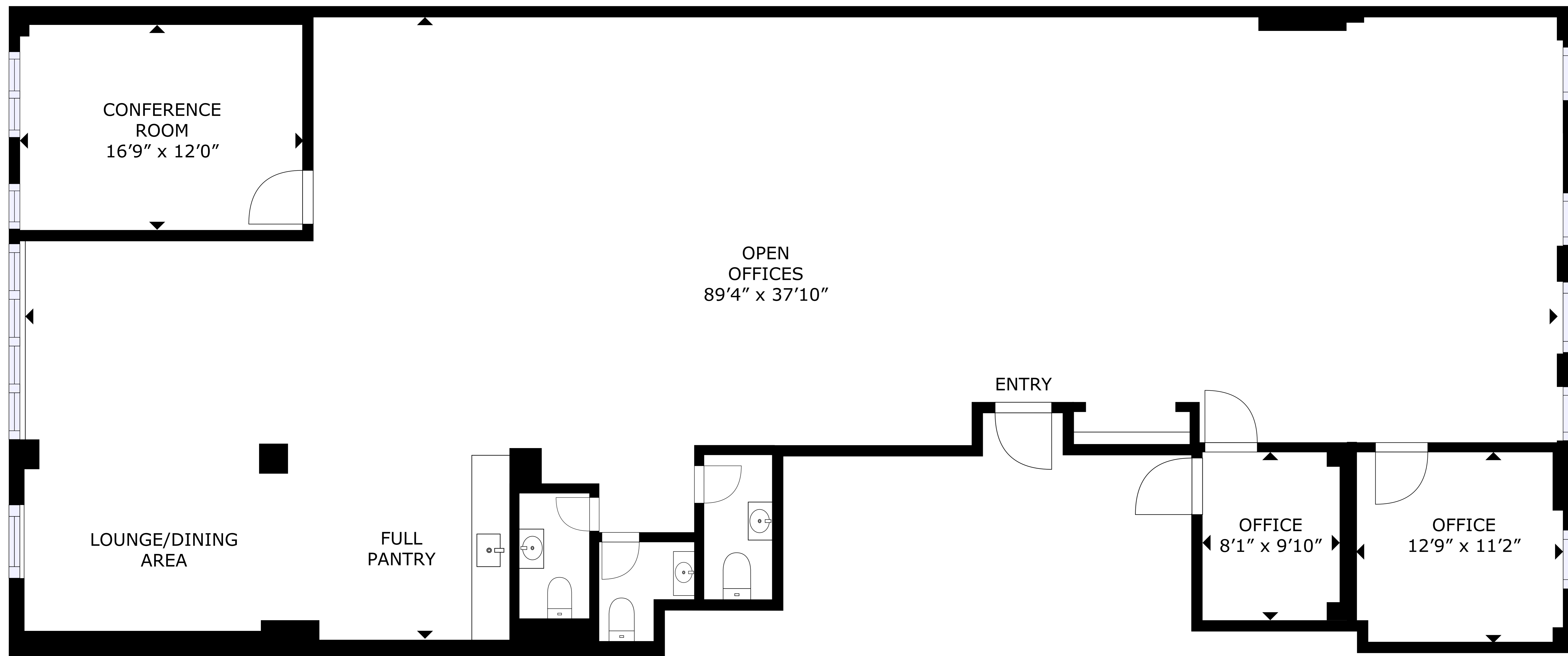
FLOOR PLAN
