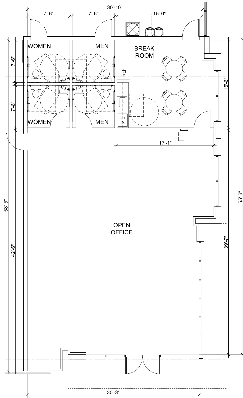
FLOOR PLAN - 1,901 SF
