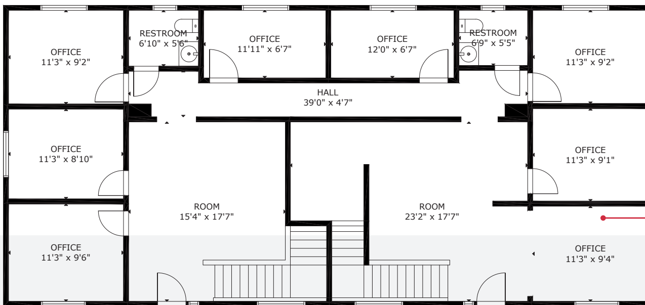
FLOOR 2
