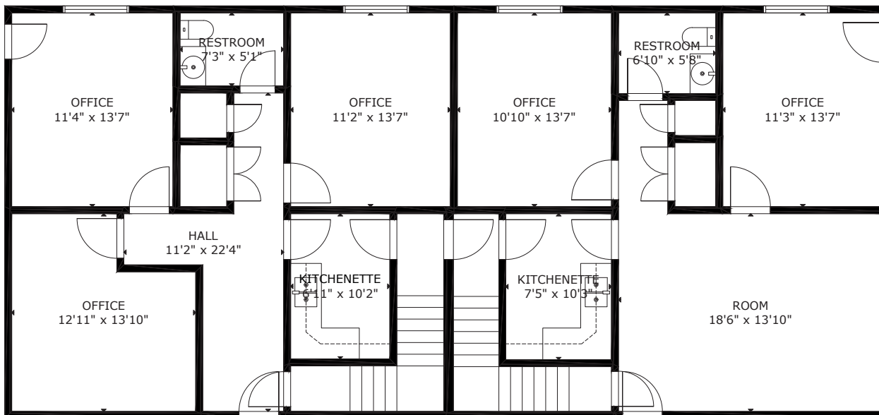
FLOOR 1
