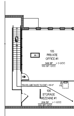
02 PROPOSED MEZZANINE FLOOR PLAN
