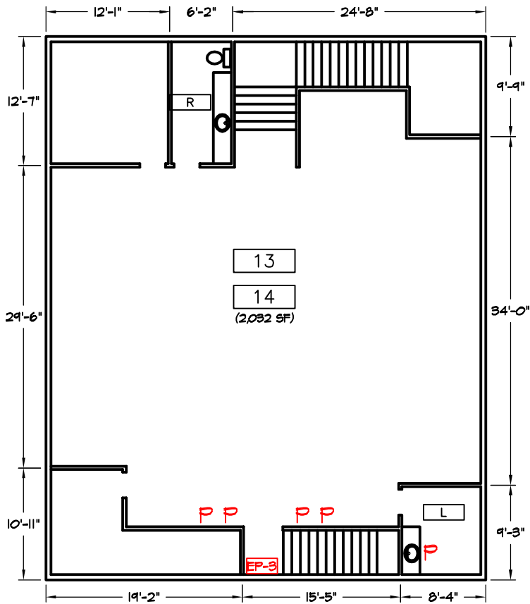
SECOND FLOOR PLAN SCALE: NONE
