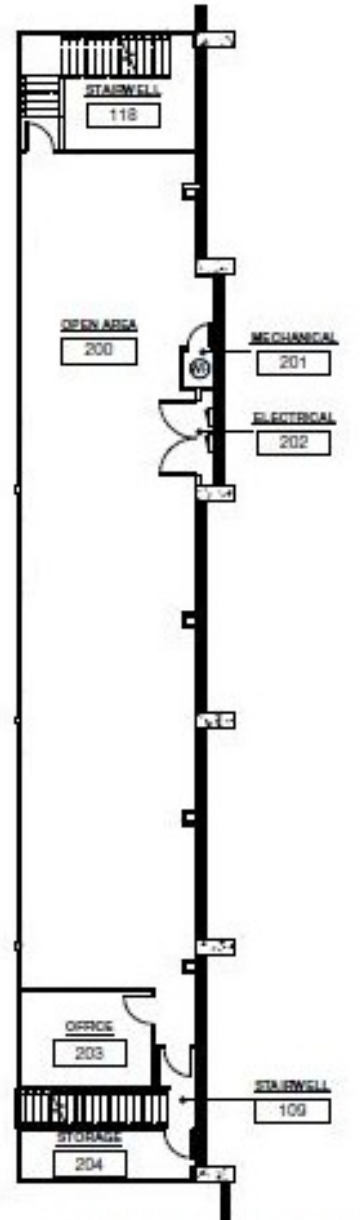
④ SUITE 200 - SECOND FLOOR (AREA D) 3/32" = 1'-0"
