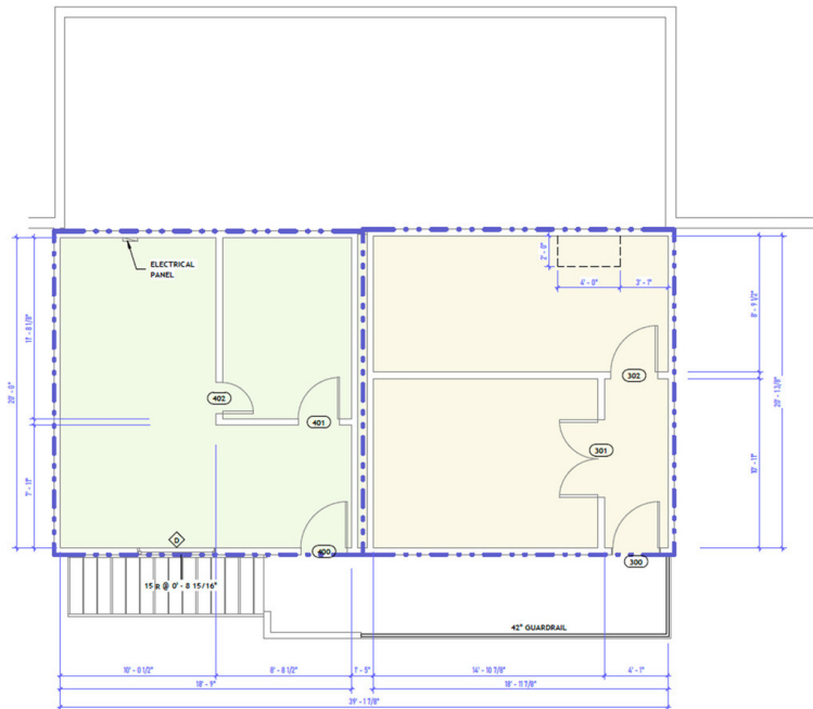
② SECOND FLOOR PLAN - OPTION 3 1/4" = 1'-0"
