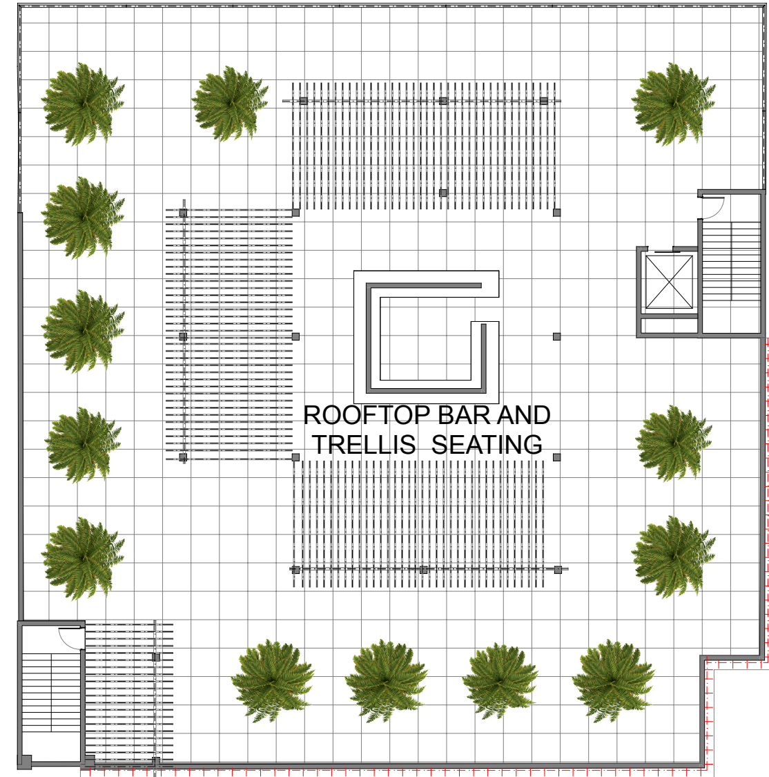
CONDO BUILDING - ROOFTOP FLOOR PLAN 10,000 SF
