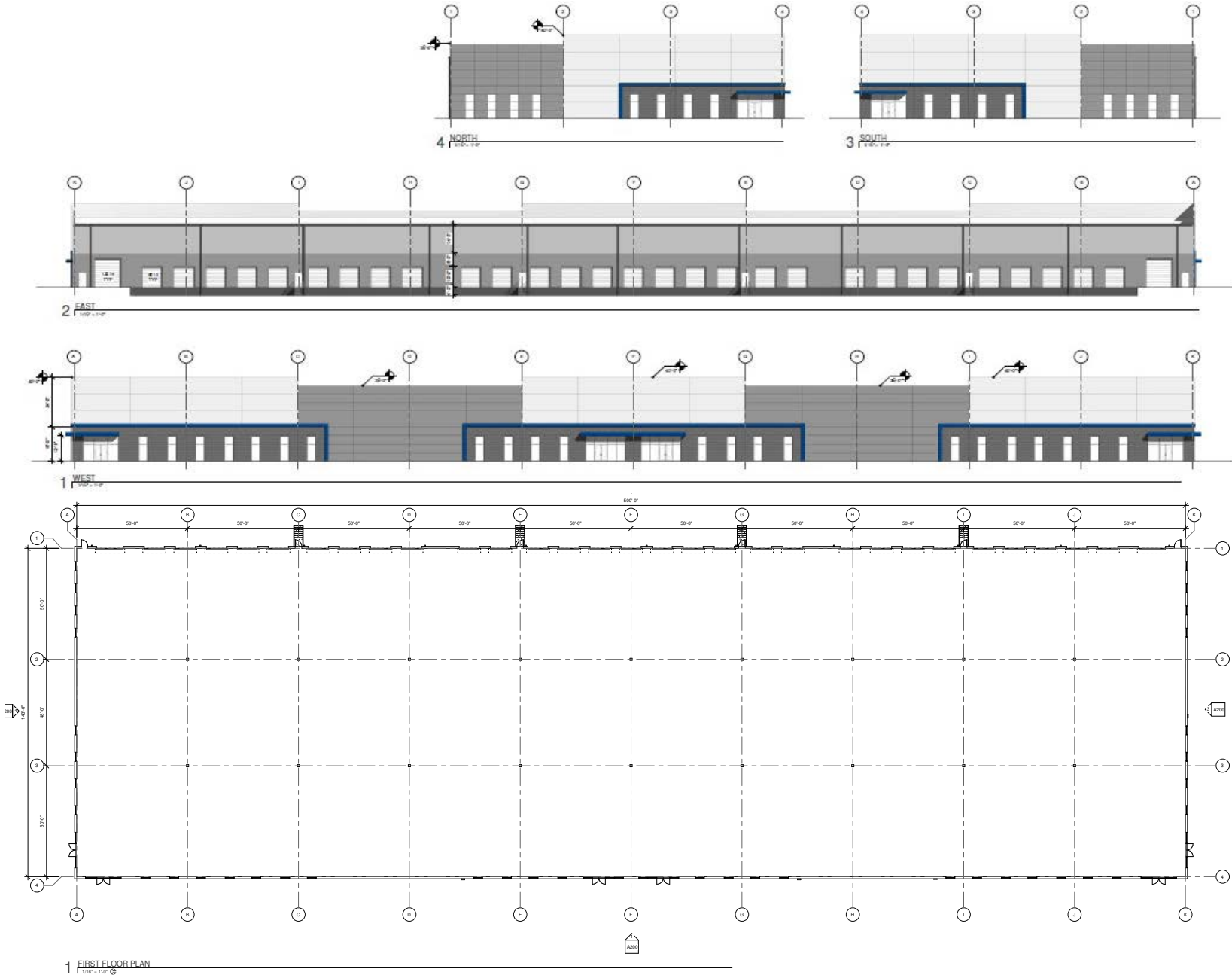
1 FIRST FLOOR PLAN 1/8" = 1'-0" G
