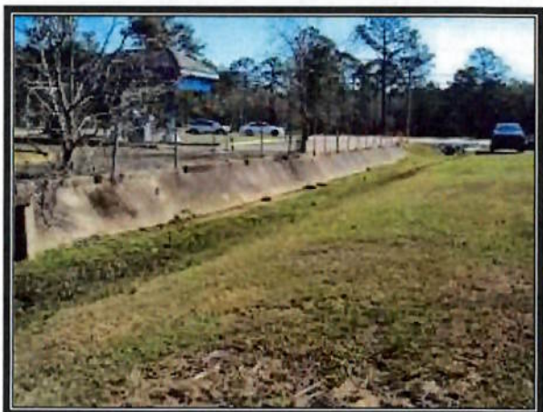
Drainage At North Property Boundary
