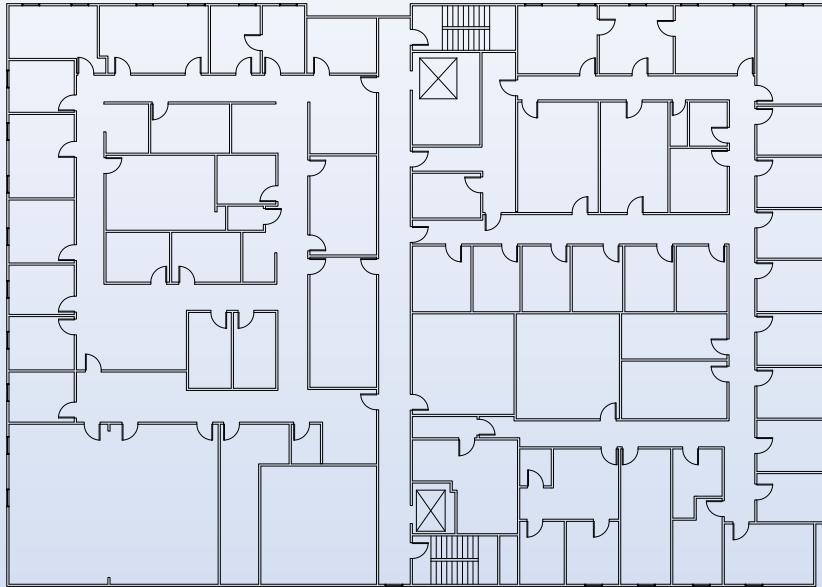
① FOURTH FLOOR PLAN 1/16" = 1'-0"
