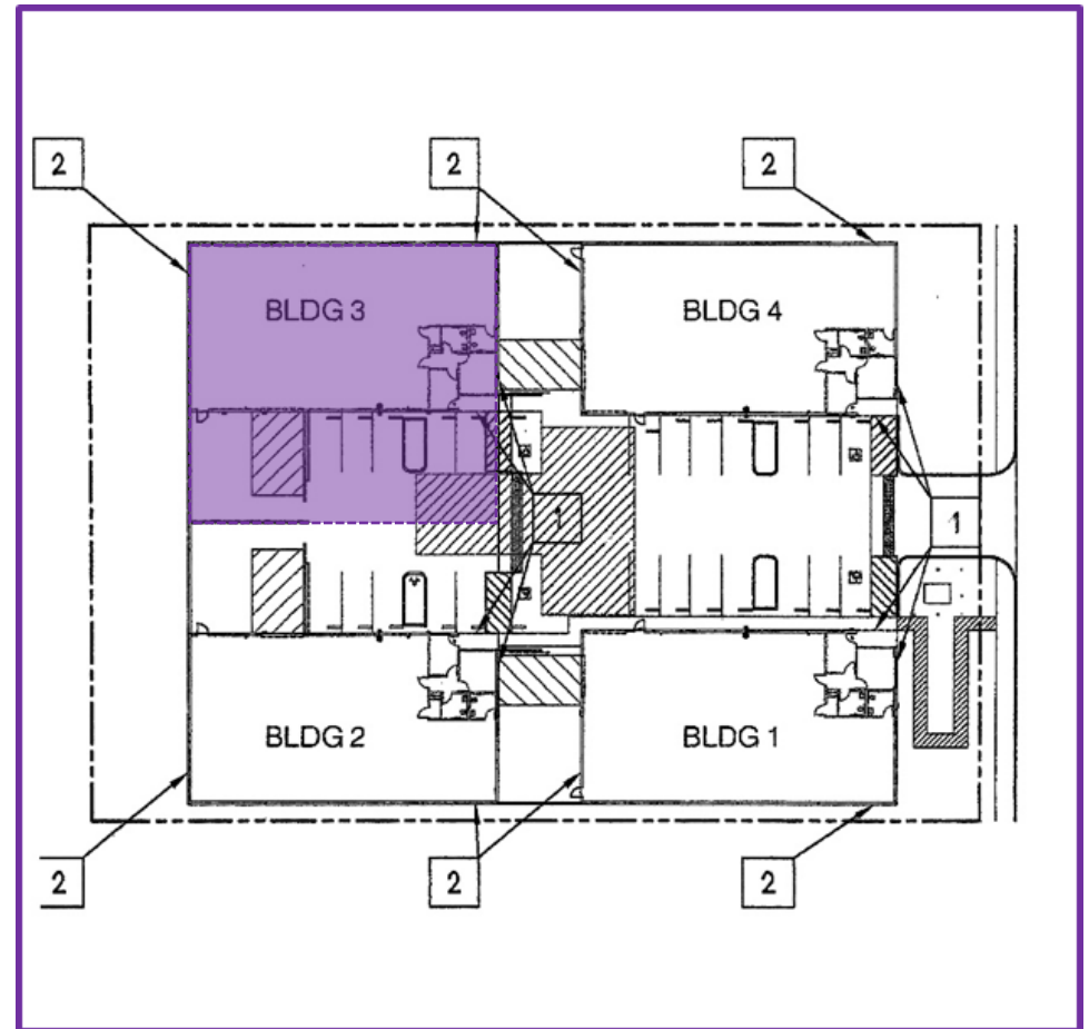
Site Plan
