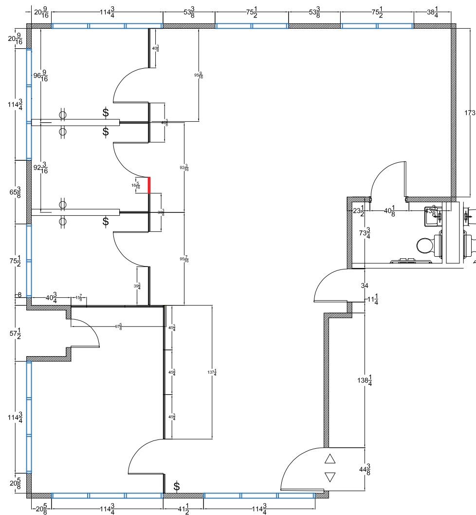
GROUND FLOOR UNIT 100
