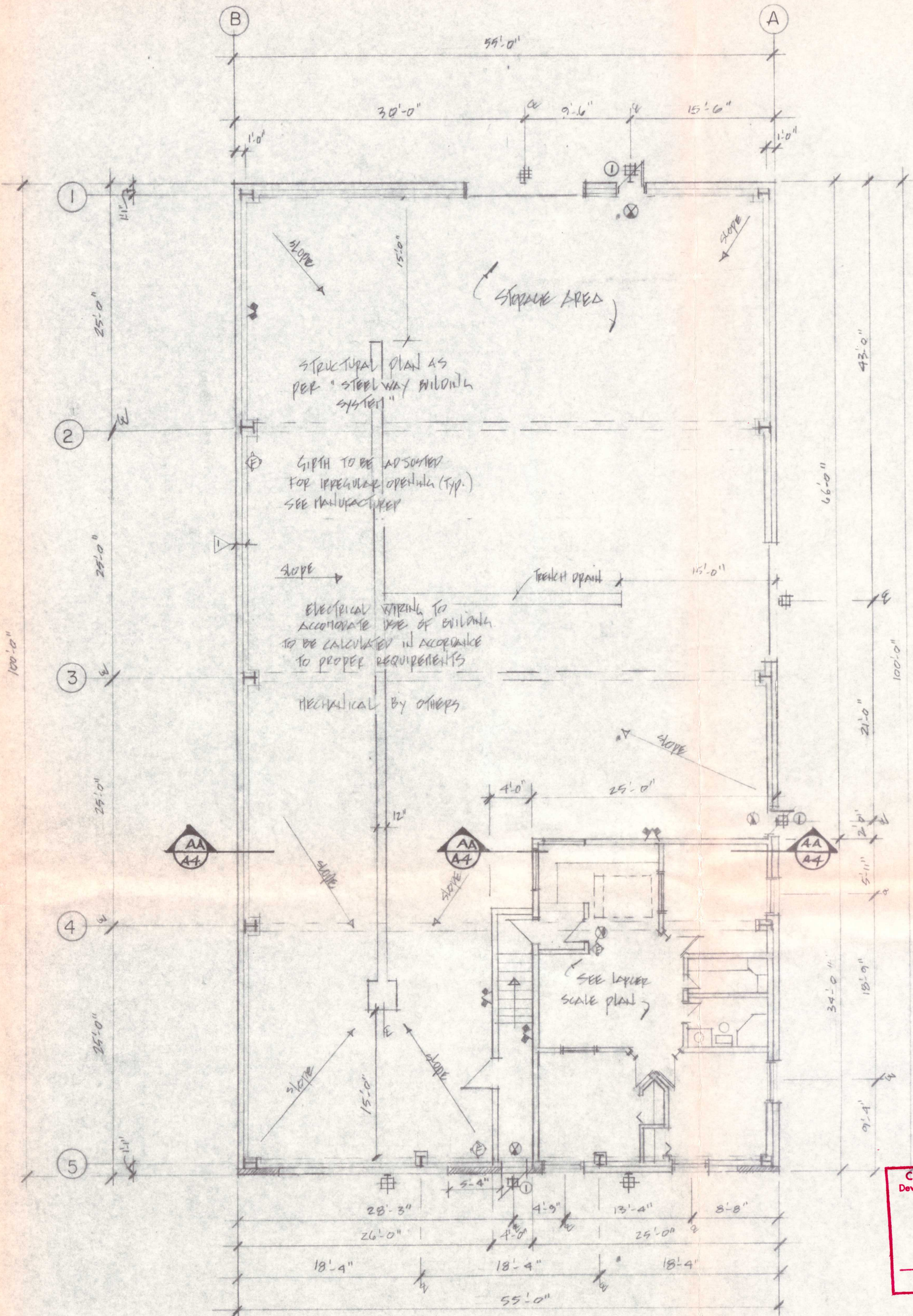
FLOOR PLAN
