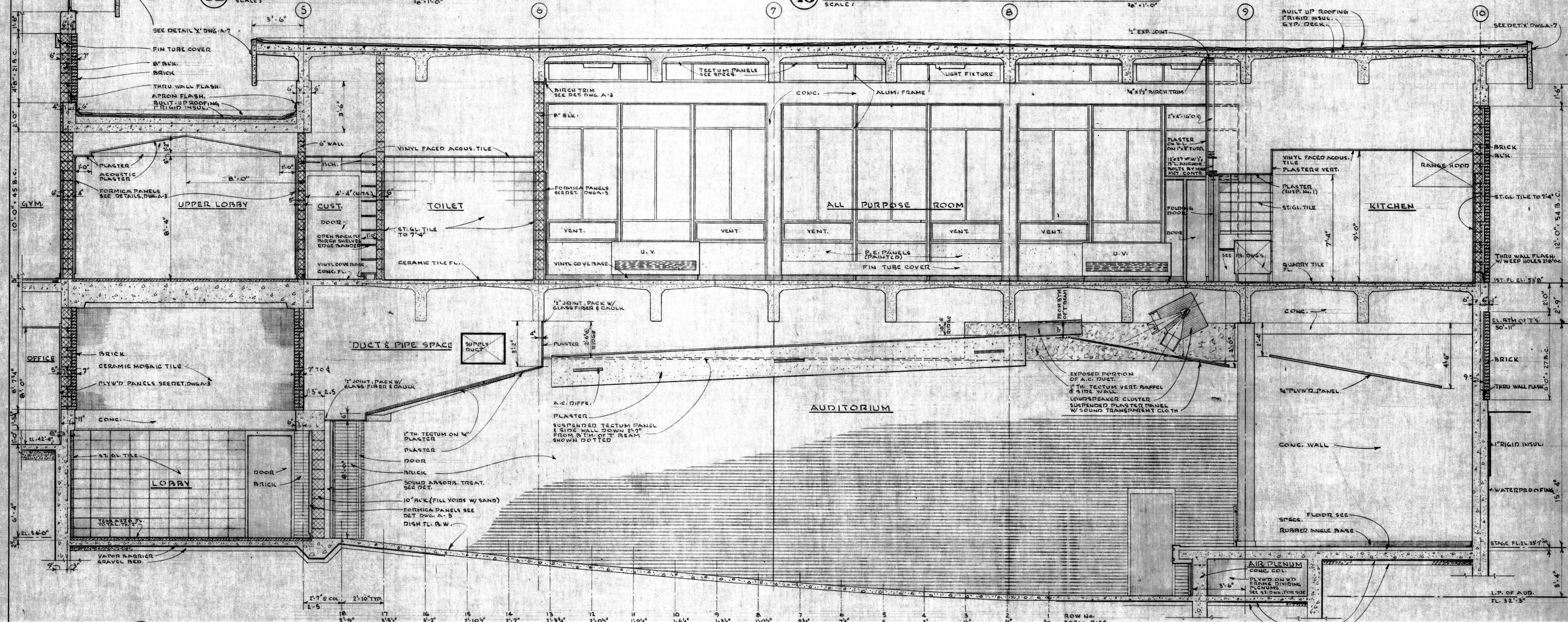
14 SECTION THRU AUD. STAGE, ALL PURPOSE ROOM, KITCHEN, LOBBY, WASHROOM & CUST. SCALE: 3/8" = 1'-0"
