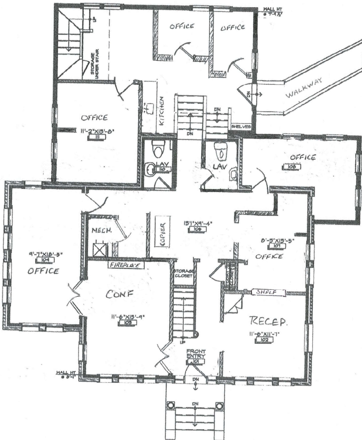
1 EXISTING CONDITIONS FIRST FLOOR PLAN SCALE: 1/8" = 1'-0" (11/16")
