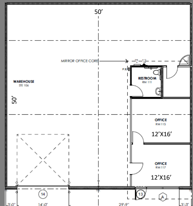
Suite Floor Plan: 101, 102, 105, 106
