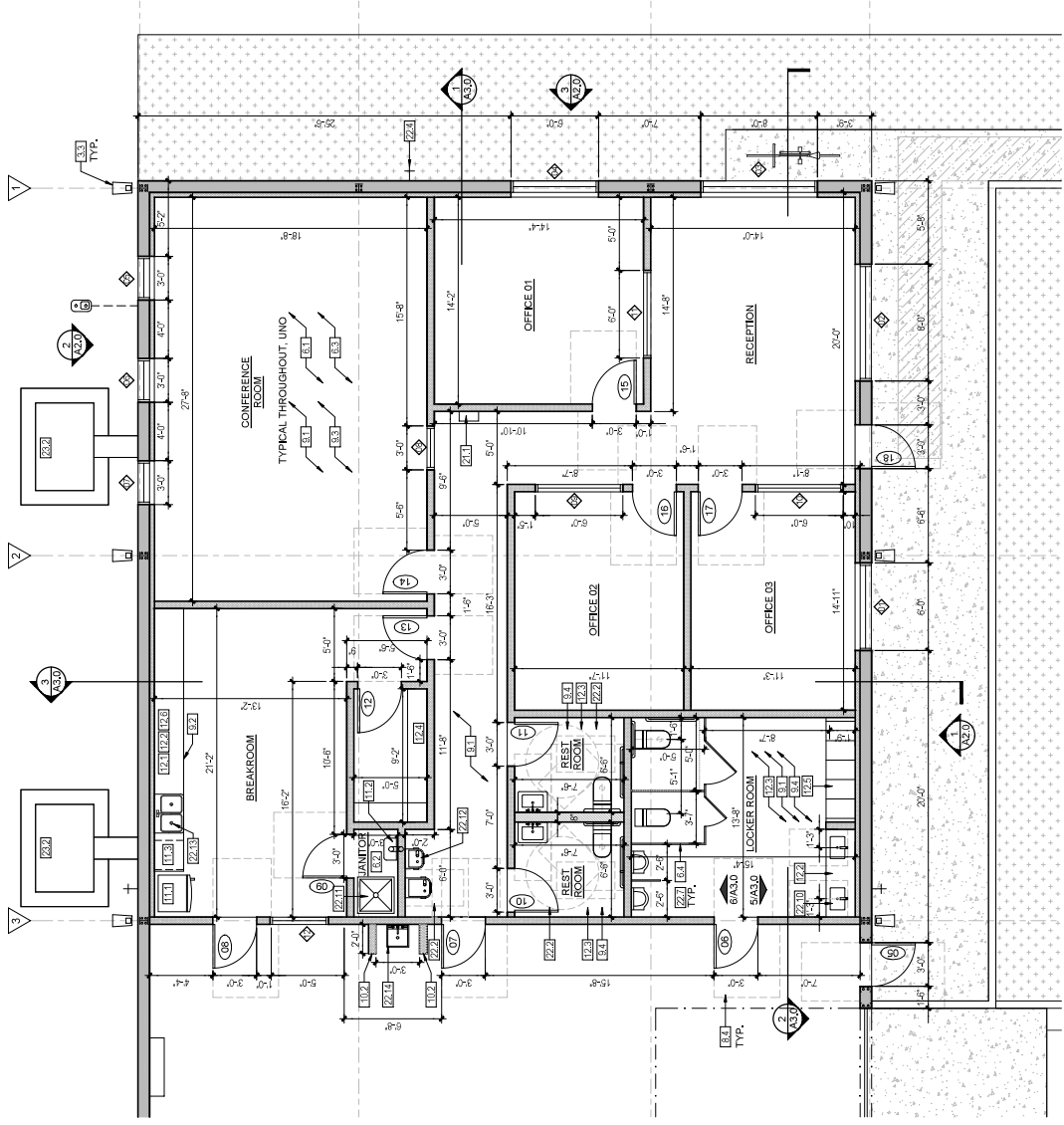
ENLARGED FLOOR PLAN SCALE: 1/4" = 1'-0"
