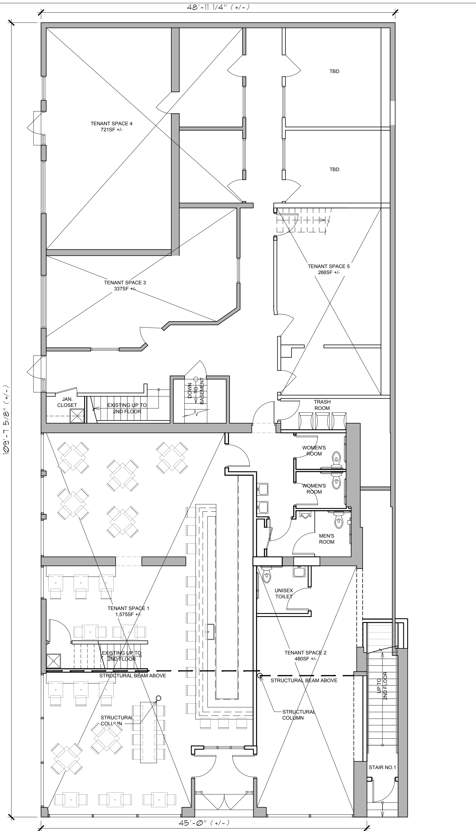
FIRST FLOOR PLAN SCALE: 1/8" = 1'-0"
