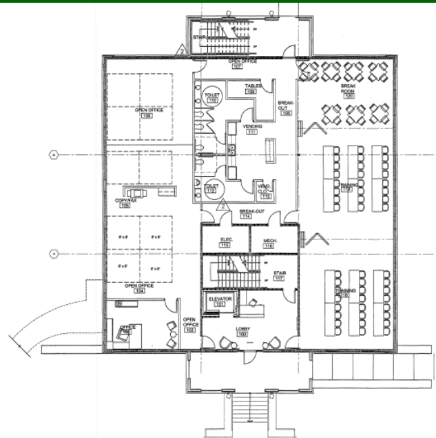
2 CONCEPTUAL SPACE PLAN-FIRST FLOOR A1.0 1/8" = 1'-0"
