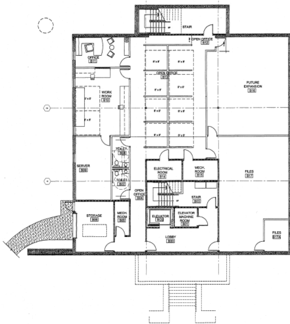
1 CONCEPTUAL SPACE PLAN-BASEMENT
