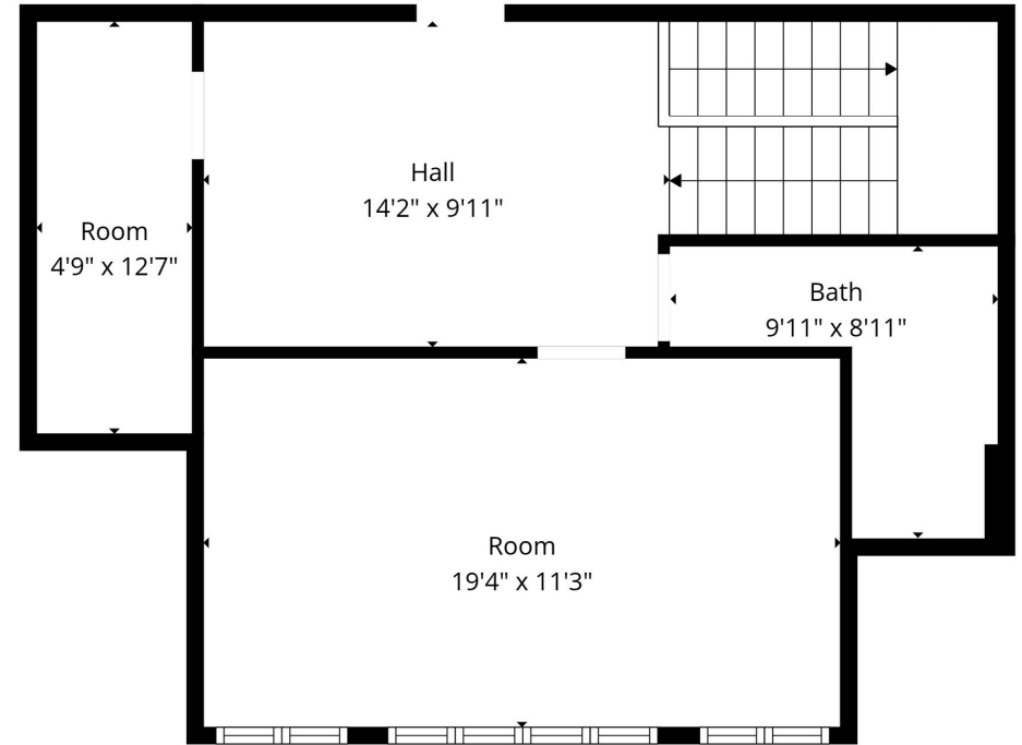
Floor 2
