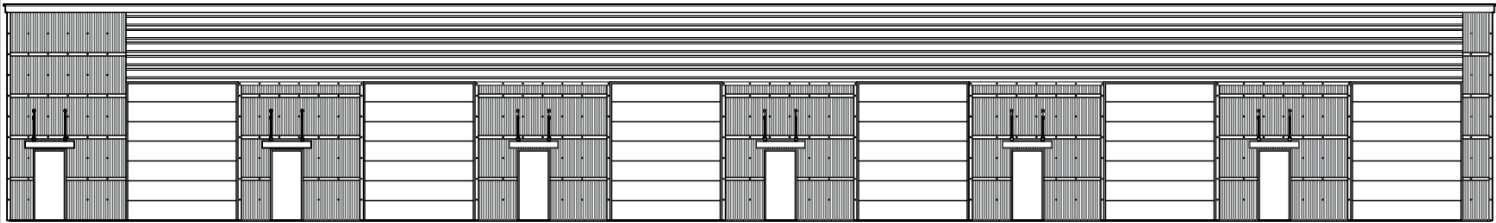
Front Elevation
