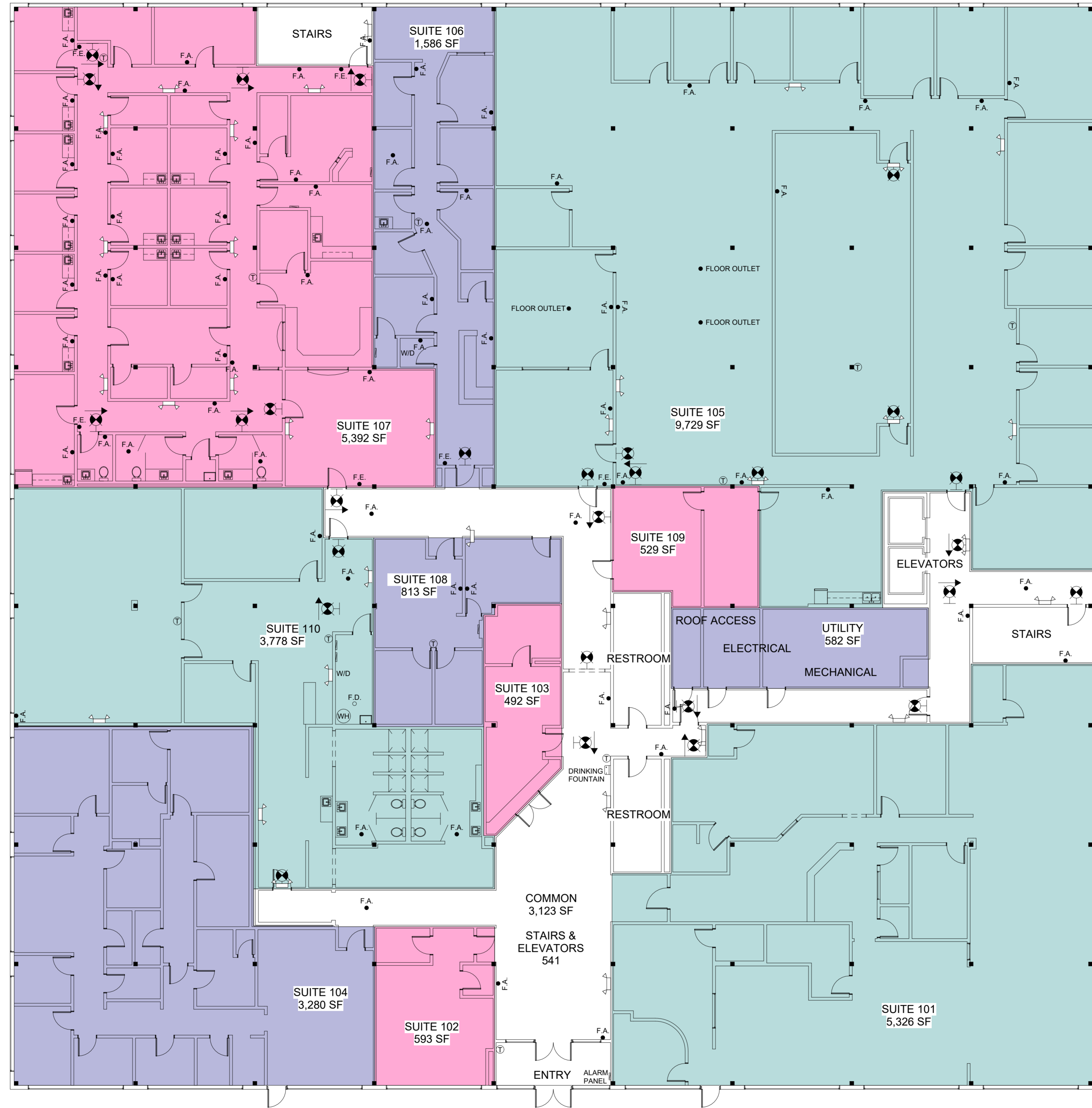
1 Level 2 Floor Plan 3/32" = 1'-0"
