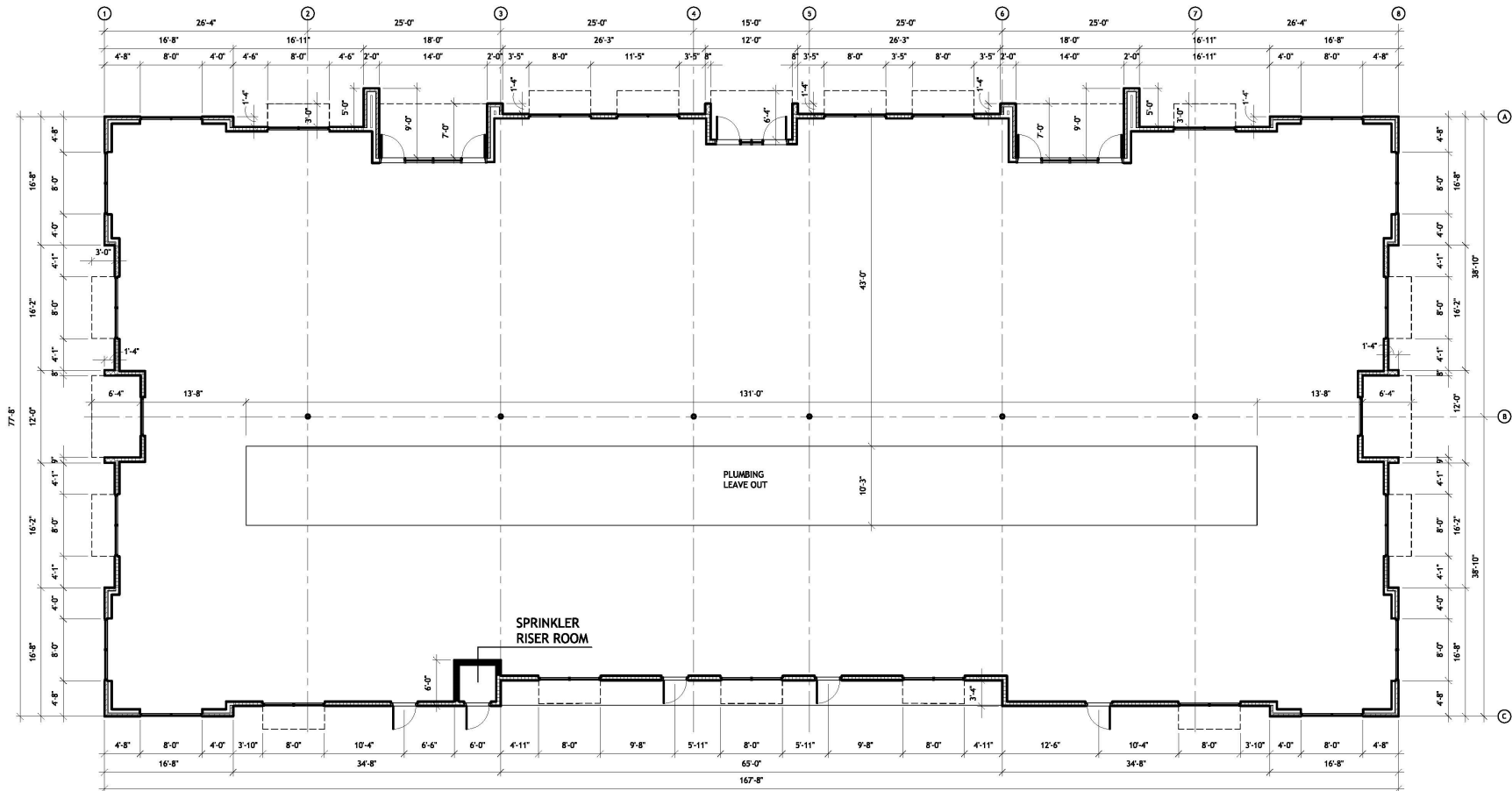
PROPOSED BUILDING "A" PLAN - 12,230 SQ. FT. (BUILDINGS "B - F" SIMILAR)
