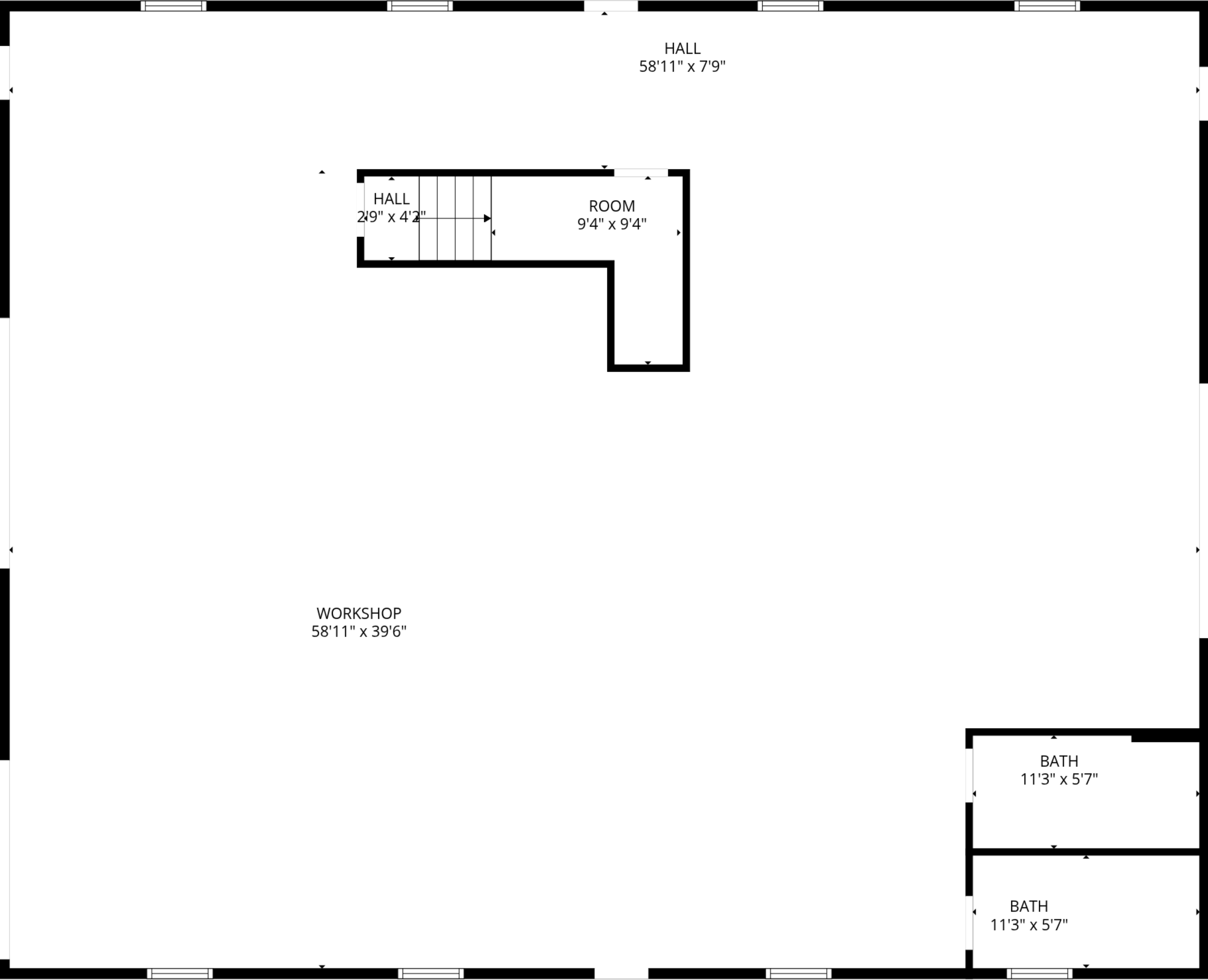
1st floor
