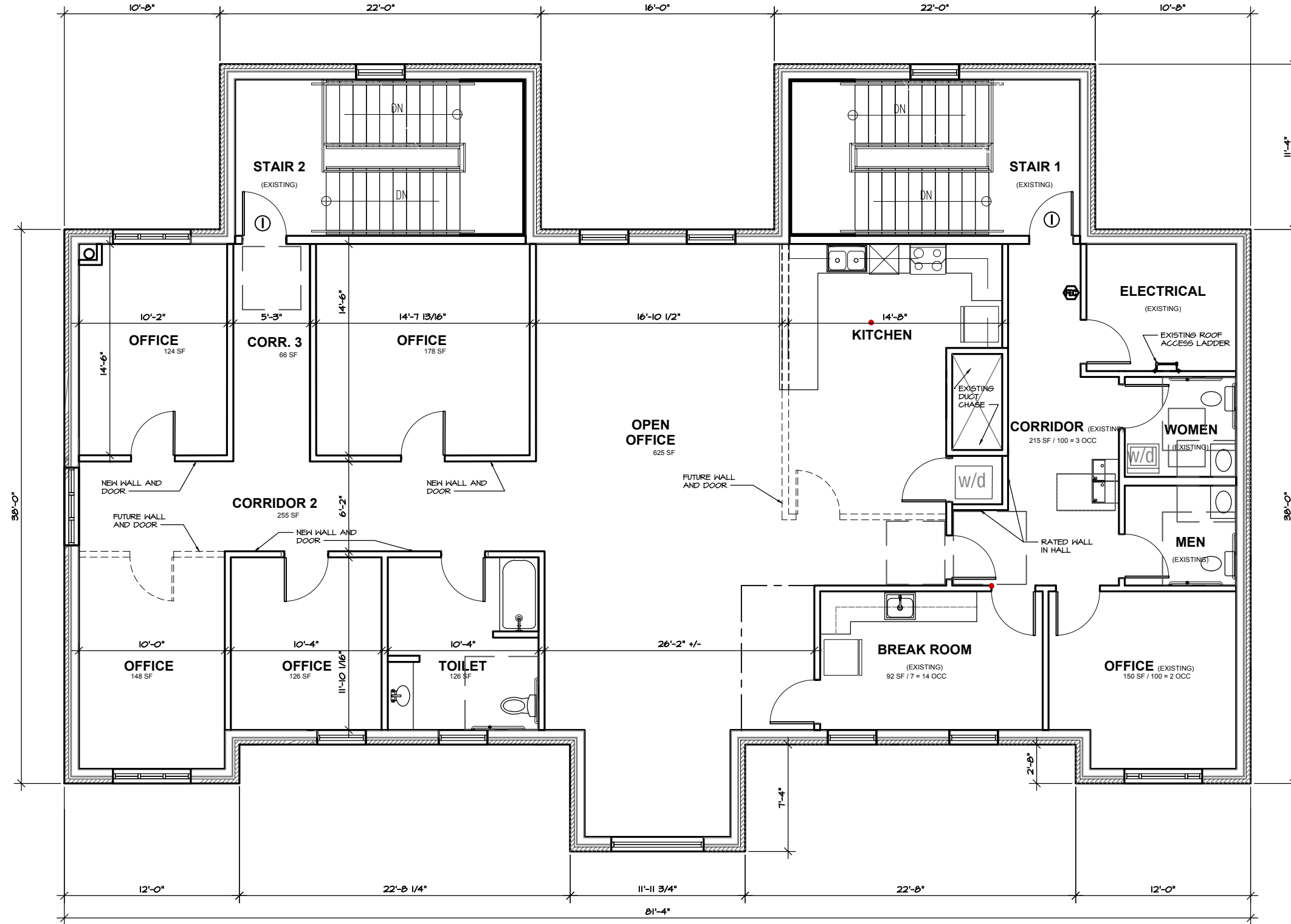
1 SECOND FLOOR PLAN AI 2893 SF 1/4"=1'-0"
