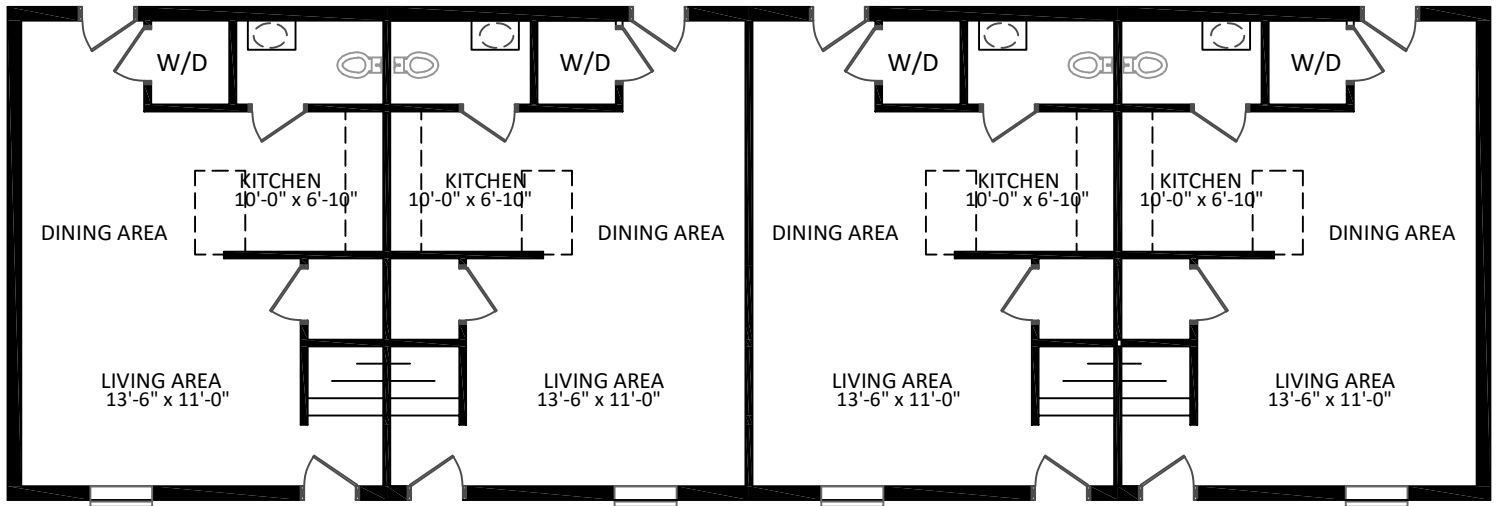
1ST FLOOR
