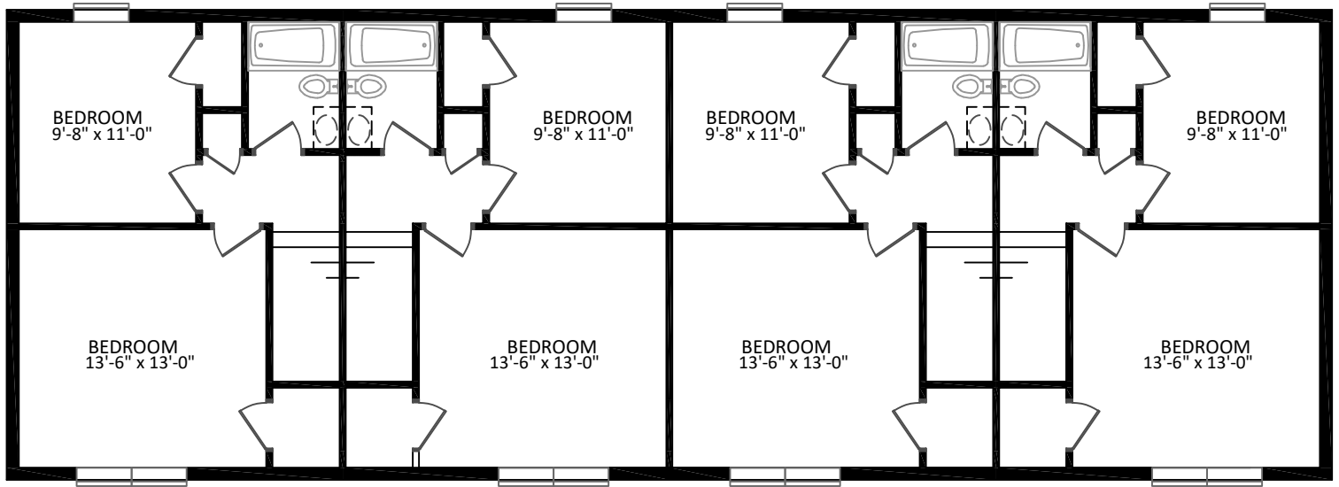
2ND FLOOR
