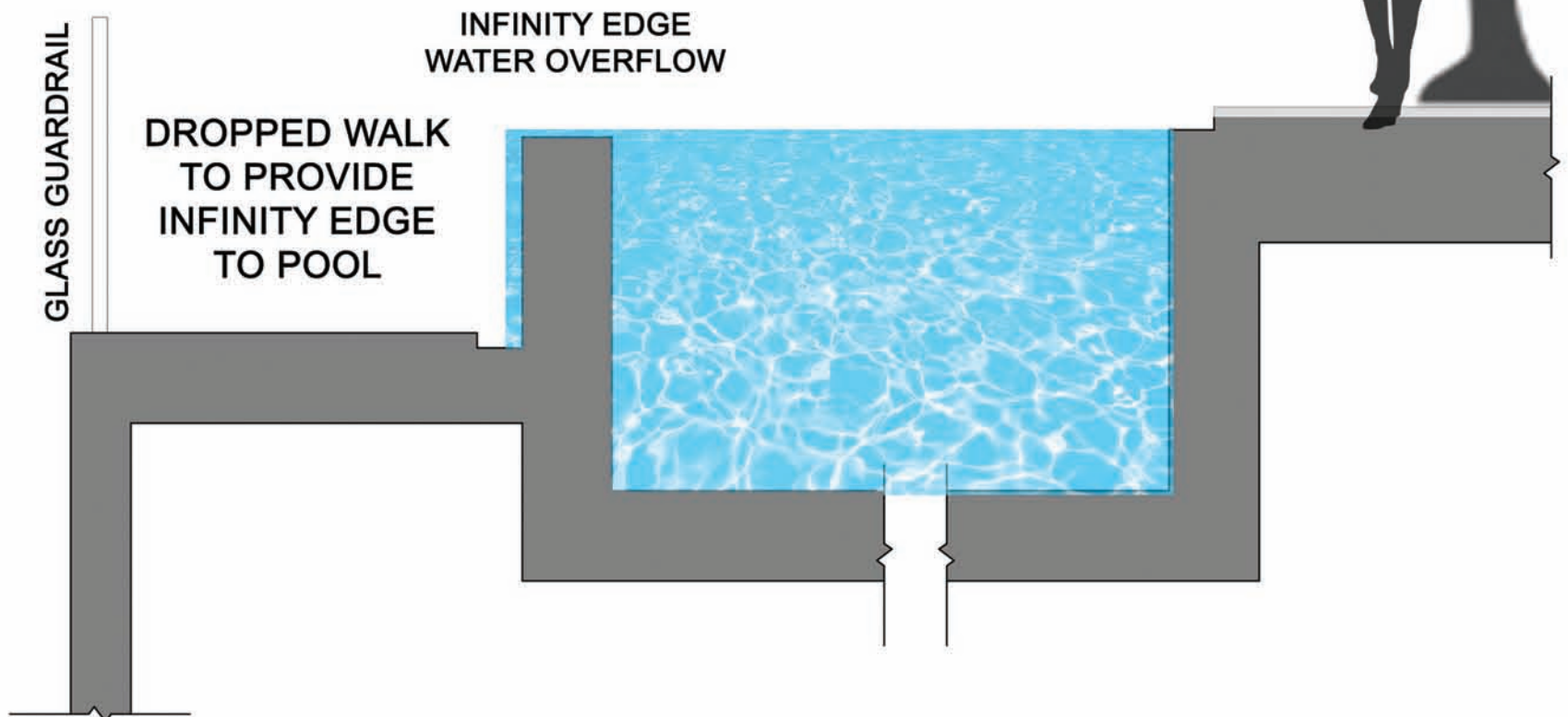
① POOL CONCEPT 1/2" = 1'-0"
