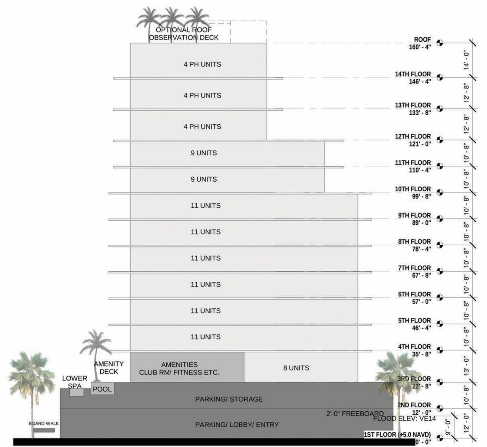
TOTAL UNITS: 104 IN 14 LEVELS SECTION ANALYSIS 1" = 20'-0"
